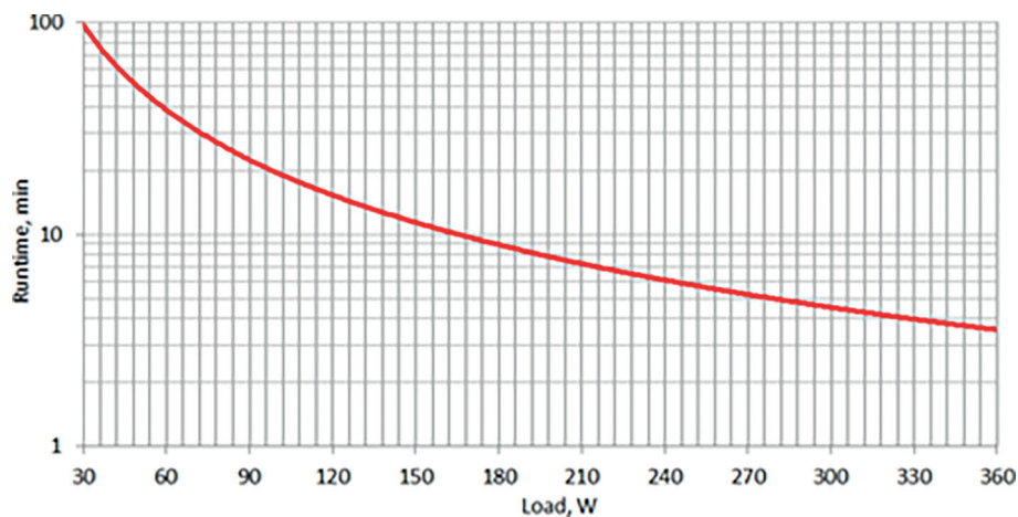
Figure 4. INFOPDU600 / INFOPDU600PL / INFOPDU600LCD autonomous operation schedule
