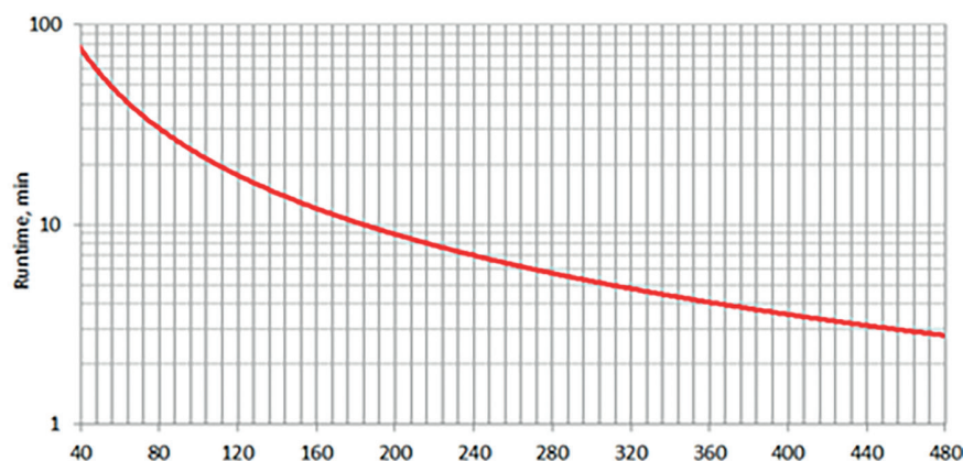
Figure 5. INFOPDU800 / INFOPDU800PL / INFOPDU800LCD autonomous operation schedule
